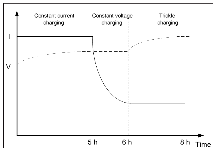
Figure 1: Optimum Charging Profile
